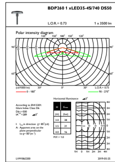
OFPL1_BDP2601xLED35-4S740DS50
