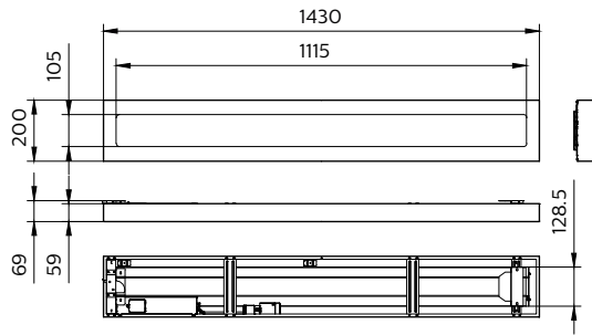
SM136V 31S_37S_43S/840 PSU W20L150 NOC
